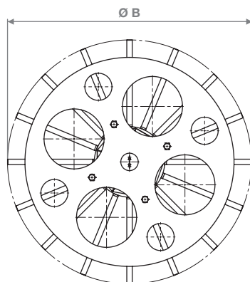
Dimensional drawing
