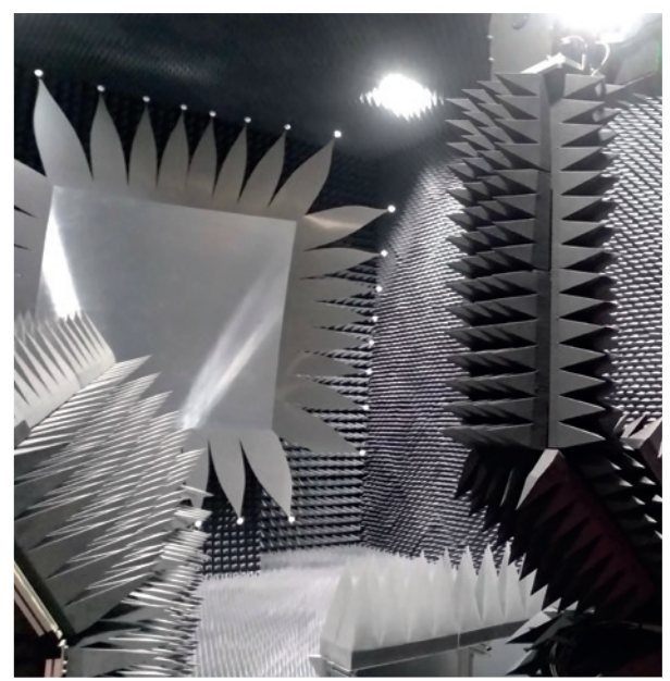
Feed, serrated-edge reflector, and positioner in a compact range
