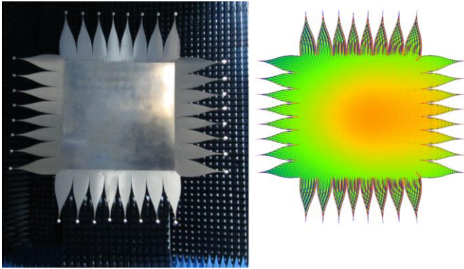
Figure 5. (Left) Orbit/FR AL-24404 single reflector with serrated edges. (Right) Plot of induced currents using MoM calculation @ 10GHz.
