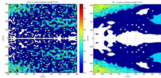
Figure 12. Predicted QZ Cx-polar discrimination @ 10 GHz. MoM and PO prediction using full wave simulation of the demonstrator and measured BFN performance. MoM analysis (left) and PO analysis (right).
