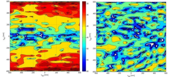
Figure 14. Contour plots of the QZ cross polar discrimination @ 11 GHz with (right) and without (left) the cross polar compensation.
