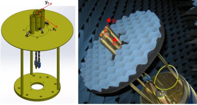
Figure 11. Mechanical model and image of the proof-of-concept demonstrator with details of the feeding network assembly.
