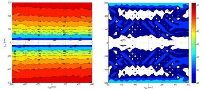
Figure 3. (Left) Example of the typical cross polar discrimination in QZ due to reflector offset. (Right) Cross polar discrimination in QZ using the proposed 3 \times 1 conjugate matched feed with optimum excitation.
