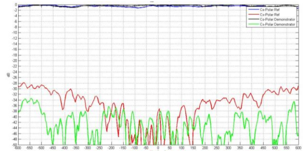
Figure 15. QZ cross polar discrimination @ 12.5 GHz. Vertical cut in the QZ with (green) and without (red) the cross polar compensation.
