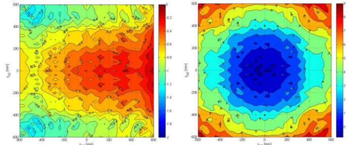
Figure 7. Co-polar amplitude and phase distribution of the QZ @ 12.5 GHz. Final 3x1 array. PO calculation and full wave array simulation.
