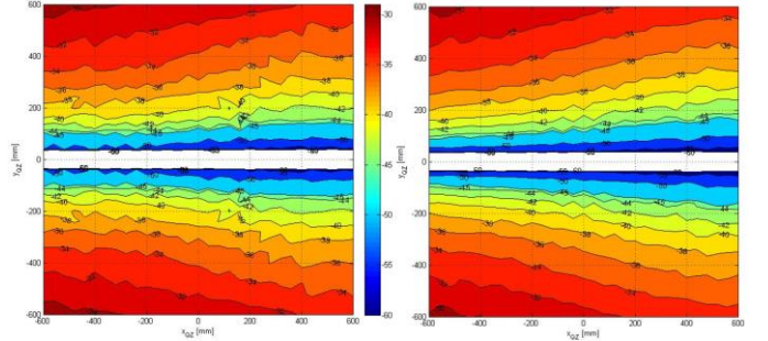
Figure 8. Cx-polar, QZ discrimination @ 12.5 GHz before compensation, Horizontal (left) and Vertical (right).
