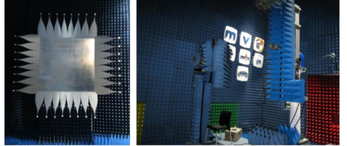
Figure 13. Orbit/FR, AL-24404, standard, side fed, single reflector CATR system installed in the Orbit facility in Israel.
