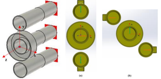
Figure 2. Conjugate matched feed array consisting of two side elements and a central element. Feed coordinate reference system with origin in the focal point. a) Side-fed CATR configuration. b) Diagonal-fed CATR configuration.
