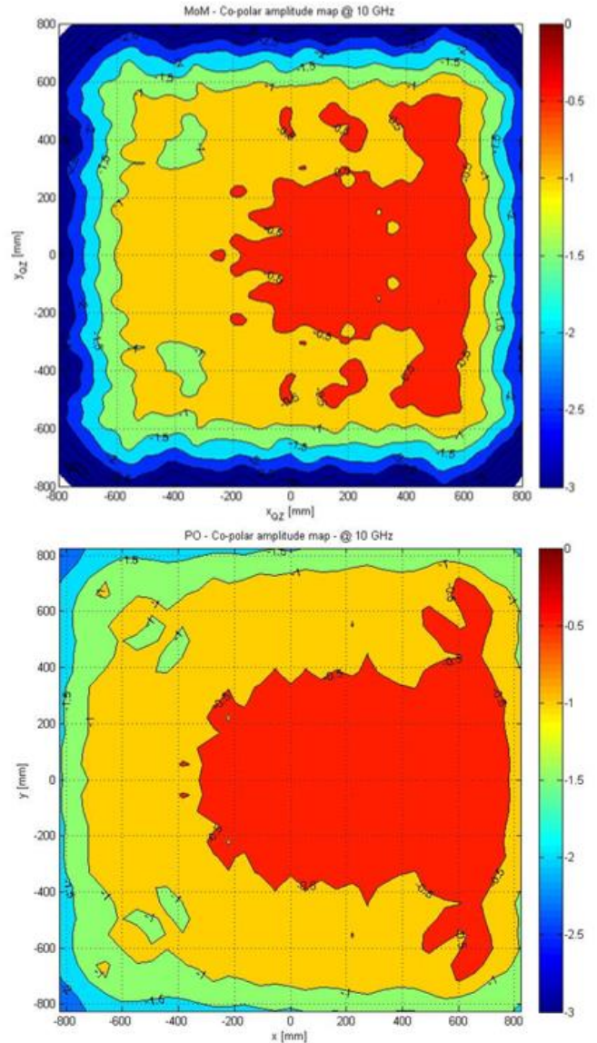
Figure 6. Performance prediction of the QZ co-polar field @ 10GHz. Full-wave MoM calculation (Top). PO approximation (Bottom)
