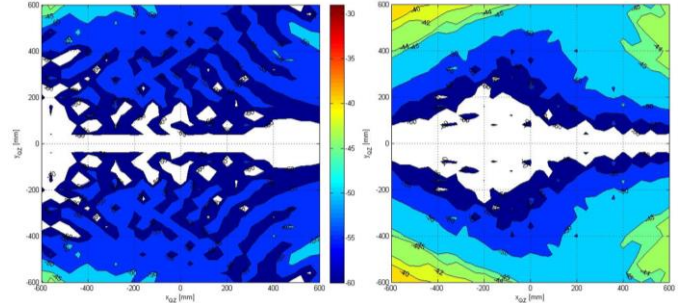
Figure 9. Cx-polar, QZ discrimination @ 10 GHz after compensation, Horizontal (left) and Vertical (right).
