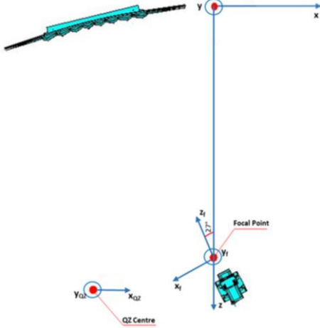
Figure 4. Relative dimensions of Orbit/FR AL-24404 single reflector, side fed, CATR with indication of feed, reflector and QZ coordinate systems.
