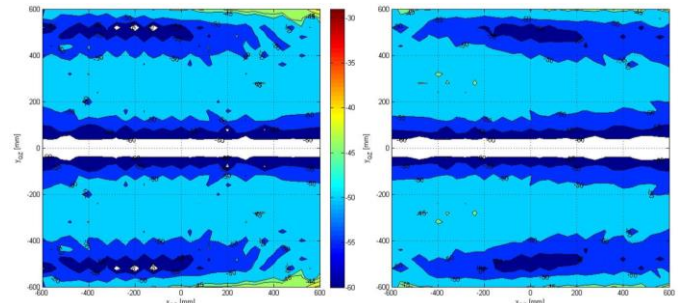
Figure 10. Cx-polar, QZ discrimination @ 15 GHz after compensation, Horizontal (left) and Vertical (right).
