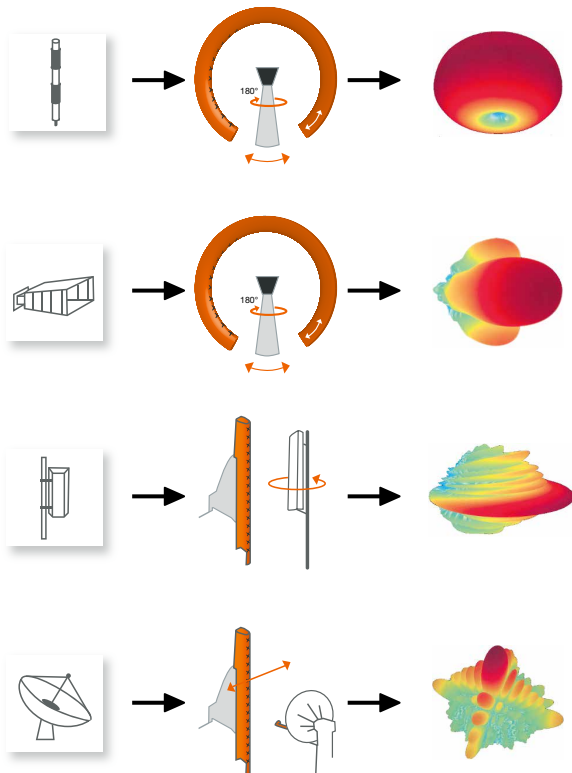
Measurement geometry according to antenna directivity
