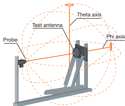
Traditional single probe spherical configuration
