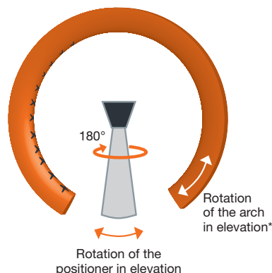
MVG's multi-probe spherical configuration
